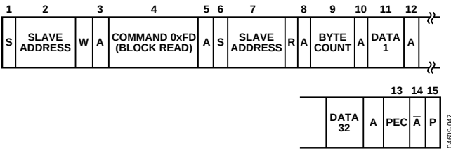
Figure 47. Block Read from EEPROM or RAM with PEC
