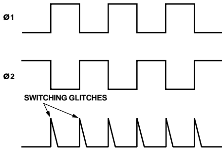
Figure 31. Switching Glitches
