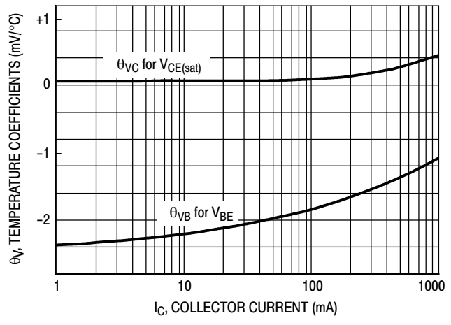
Figure 4. Temperature Coefficients
