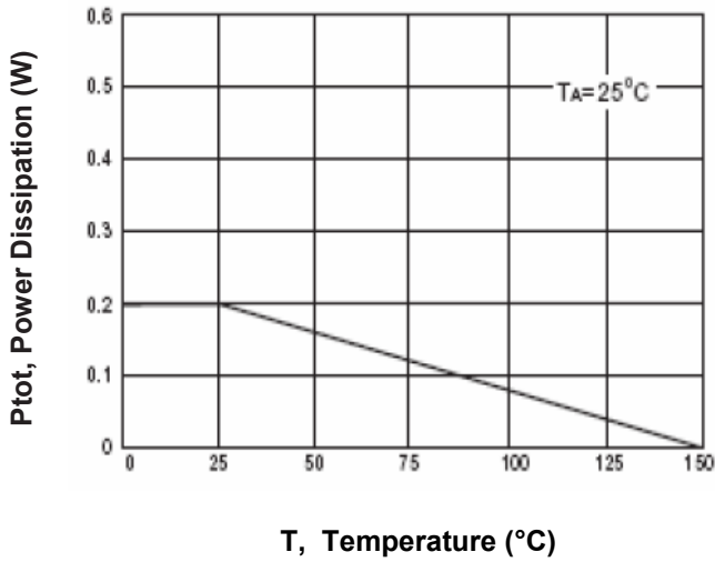
Fig.1- Power Dissipation
