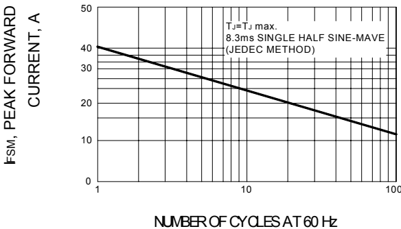
FIG.6 – MAXIMUM NON-REPETITIVE FORWARD SURGE CURRENT UNIDIRECTIONAL ONLY
