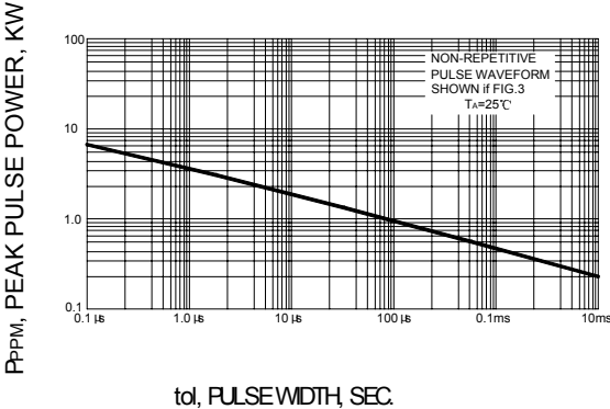
FIG.3 – PULSE WAVEFORM
