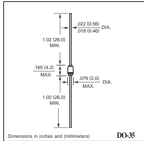
DO-35
