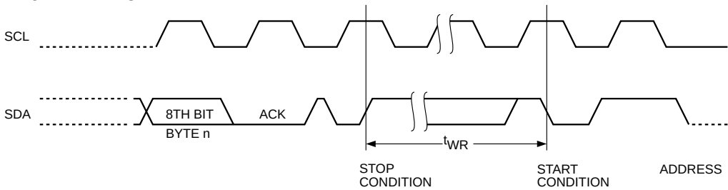
Figure 3. Start/Stop Timing
