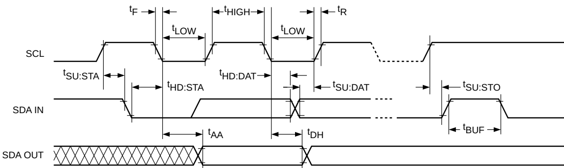
Figure 1. Bus Timing
