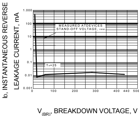
FIG.7 – TYPICAL REVERSE LEAKAGE CHARACTERISTICS
