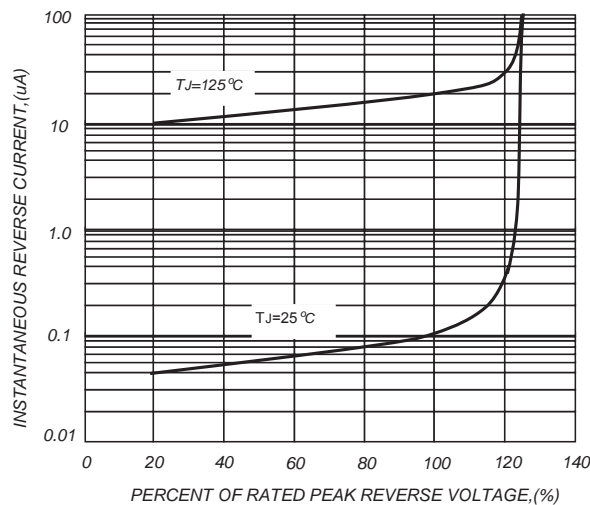
FIG.5-TYPICAL REVERSE CHARACTERISTICS
