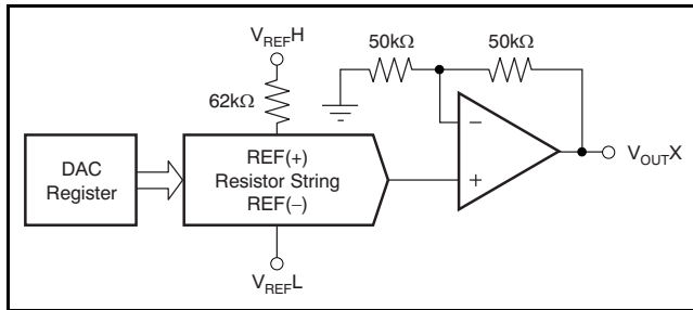
Figure 92. DAC7565 Architecture
