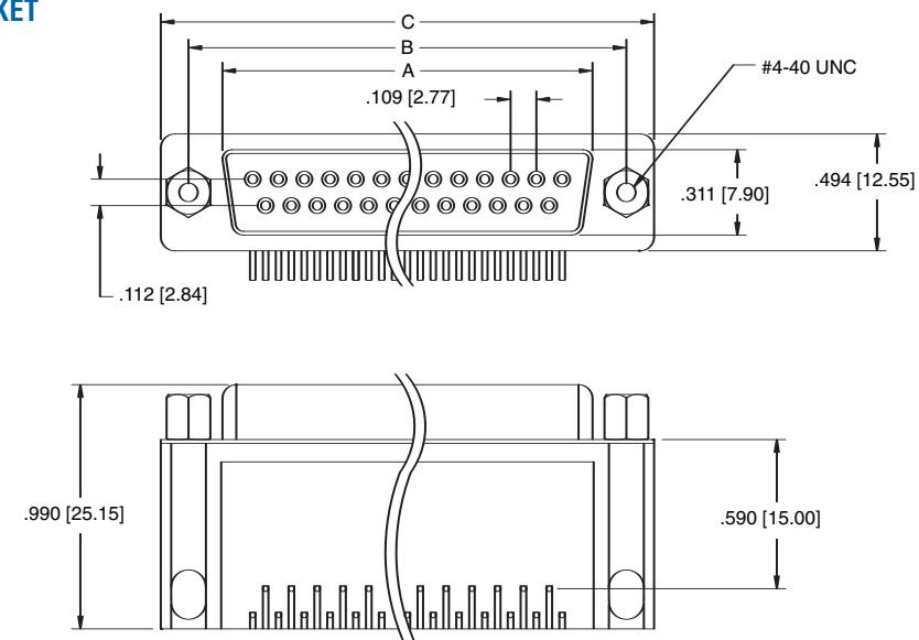
DB25-SQ-R5
