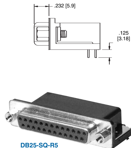
DB25-SQ-R5
