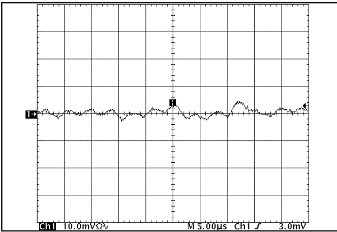
Figure 19: Input Reflected Ripple Current, i_s , through a 10 \mu H source inductor at nominal input voltage and rated load current (5 mA/div). 1.5V and 3.3V outputs at full rated load current. (see Fig. 17)
