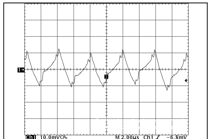
Figure 18: Input Terminal Ripple Current, 1.5V & 3.3V outputs at full rated output current and nominal input voltage with 10 \mu H source impedance and 100 \mu F electrolytic capacitor (10 mA/div). (see Fig. 17)
