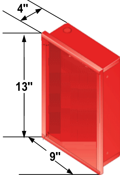
Figure 1 Backbox Dimensions
