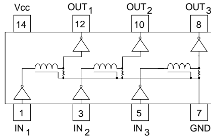
Triple 14-Pin Schematic
