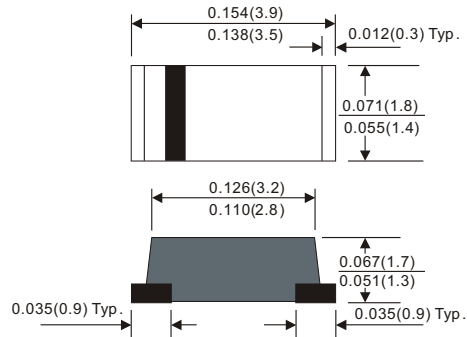
SOD-123
