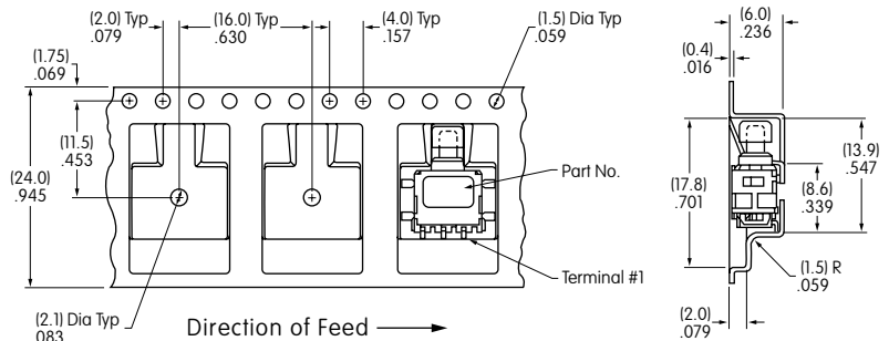
Tape Dimensions
