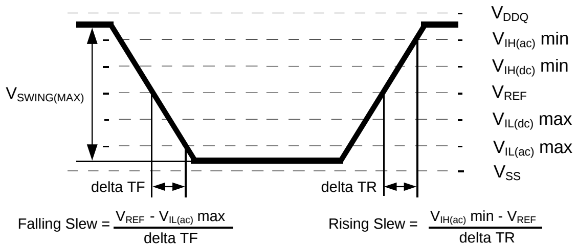
< Figure : AC Input Test Signal Waveform >
