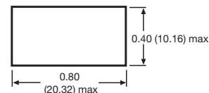
DIP Package
