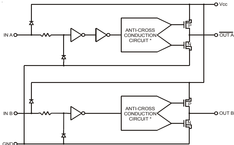
Figure 3 - IXDF404 Inverting + Non-Inverting 4A Gate Driver Functional Block Diagram
