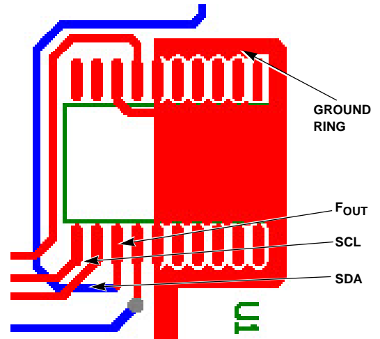
FIGURE 21. SUGGESTED LAYOUT FOR THE ISL12022M
