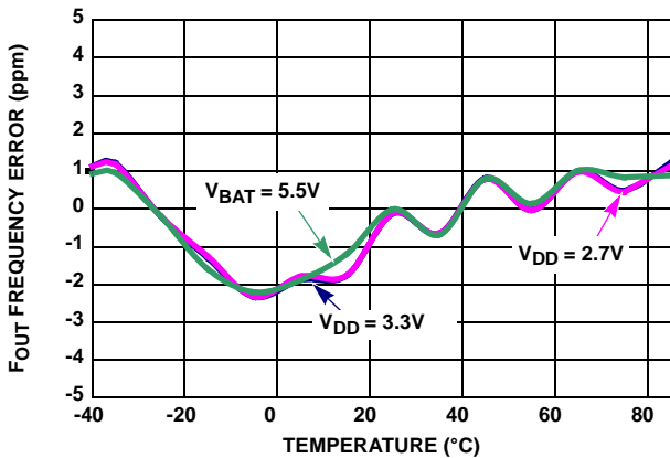
FIGURE 6. OSCILLATOR ERROR vs TEMPERATURE
