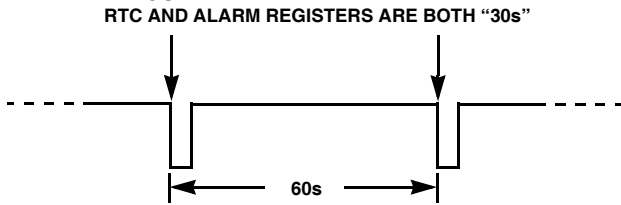
FIGURE 14. \overline{\text{IRQ}}/\text{F}_{\text{OUT}} WAVEFORM
