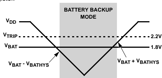
FIGURE 12. BATTERY SWITCHOVER WHEN V_{BAT} < V_{TRIP}
