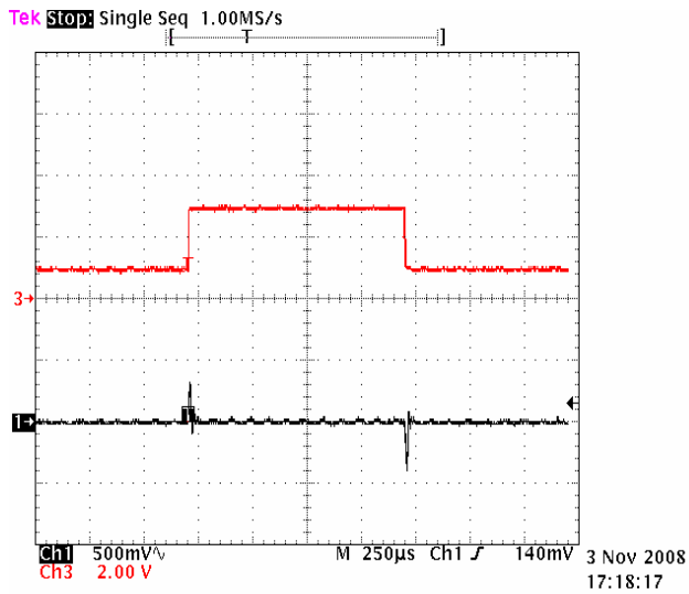
FIGURE 59. LOAD TRANSIENT RESPONSE, 100nF LOAD CAPACITANCE
