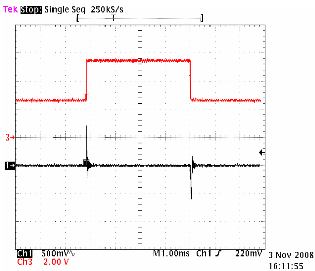
FIGURE 61. LINE TRANSIENT RESPONSE, 100nF
