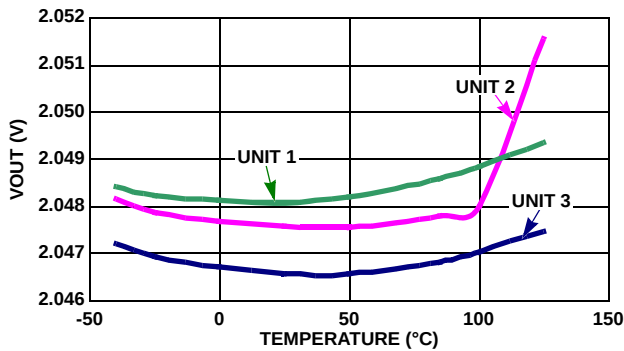
FIGURE 47. V_{OUT} vs TEMPERATURE, 3 UNITS
