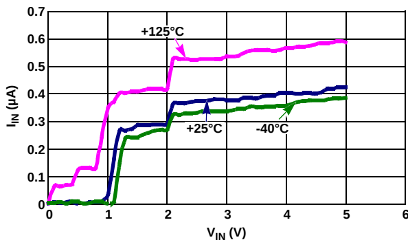
FIGURE 49. I_{IN} vs V_{IN} [SLEEP MODE], 3 TEMPERATURES
