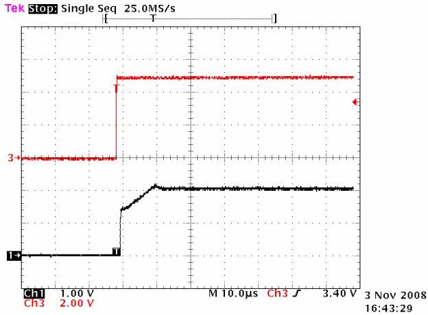
FIGURE 57. TURN-ON TIME, 1k \Omega
