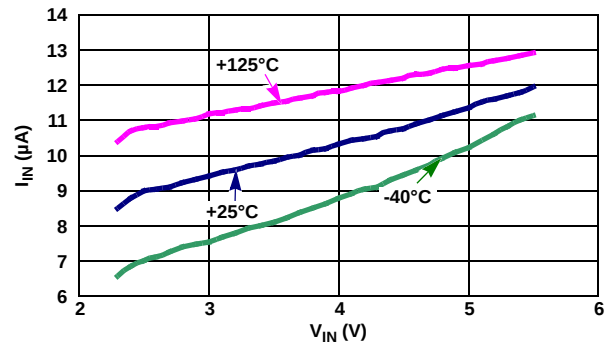
FIGURE 48. I_{IN} vs V_{IN} , 3 TEMPERATURES
