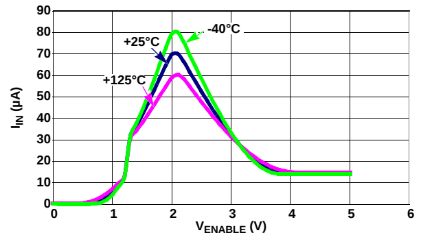
FIGURE 36. I_{IN} vs V_{ENABLE} , 3 TEMPERATURES
