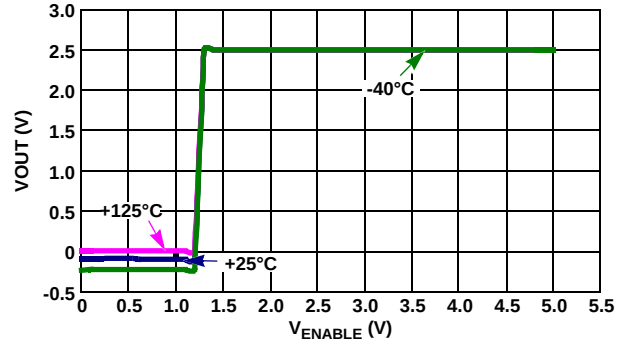
FIGURE 46. V_{OUT} vs V_{ENABLE}
