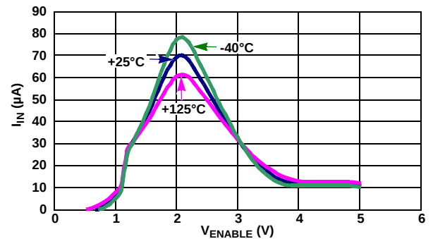
FIGURE 50. I_{IN} vs V_{ENABLE} , 3 TEMPERATURES
