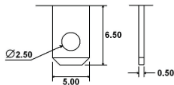
Solder Tabs
