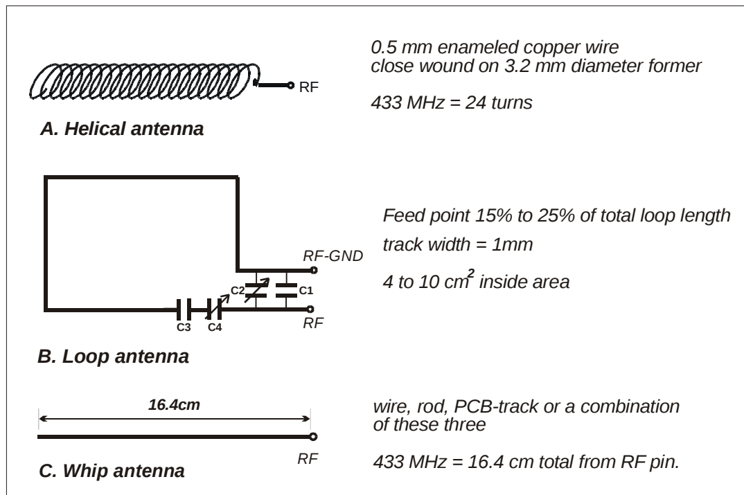
Figure 6: Antenna
