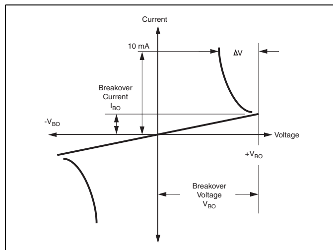
V-I Characteristics
