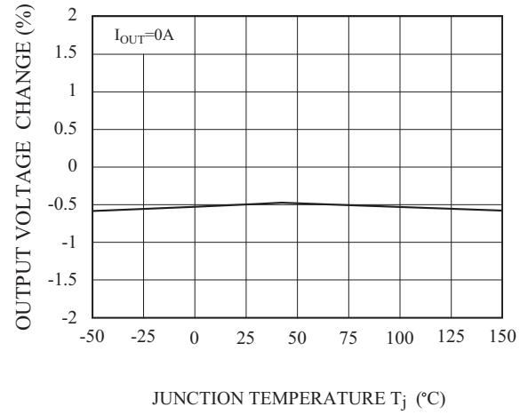
Fig. 4 V_{OUT}(\text{CHANGE}) - T_j
