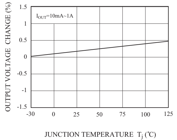
Fig. 4 LOAD REGULATION
