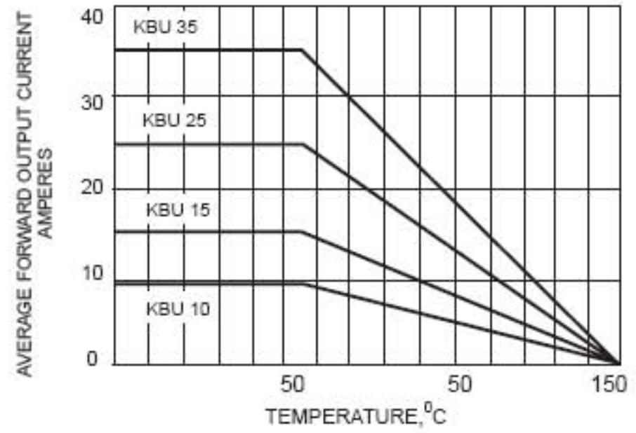
FIG.2 -DERATING CURVE OUTPUT RECTIFIED CURRENT
