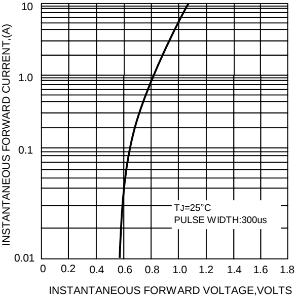
FIG.4-TYPICAL FORWARD CHARACTERISTICS
