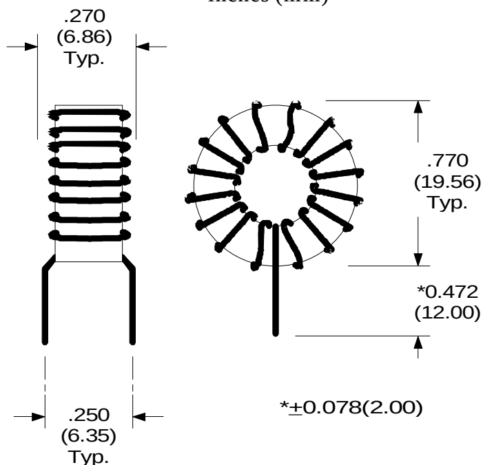
Physical Dimensions inches (mm)
