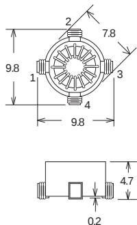
Bottom View
