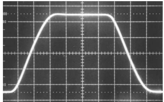
Figure 17. Drive Output Rise and Fall Time
