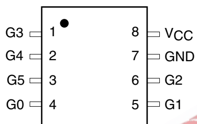
Figure 10: ACE1101 Pinout – Normal Operation
