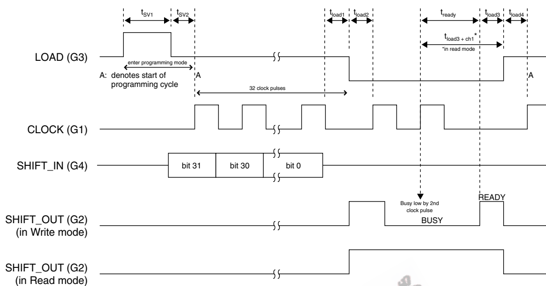
Figure 22: Programming Protocol
