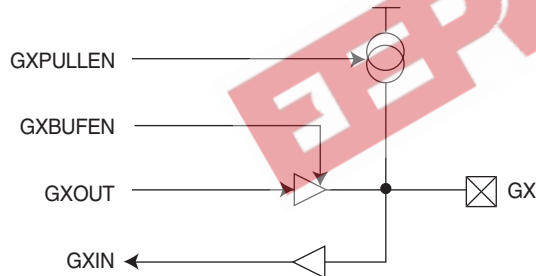
Figure 28. PORTGD Logic Diagram
