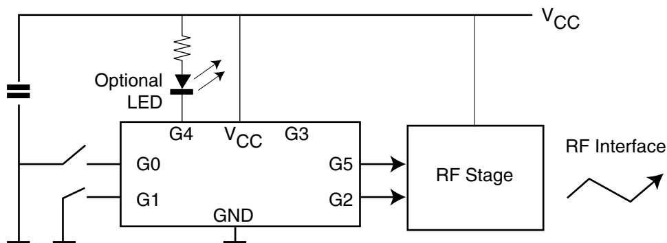
Figure 2: ACE Ex Application Example (Remote Keyless Entry)
