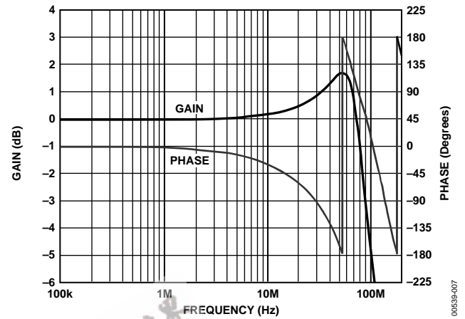
Figure 7. Frequency and Phase Response vs. Gain (Gain = +10\text{ dB} , P_{IN} = -30\text{ dBm} )
