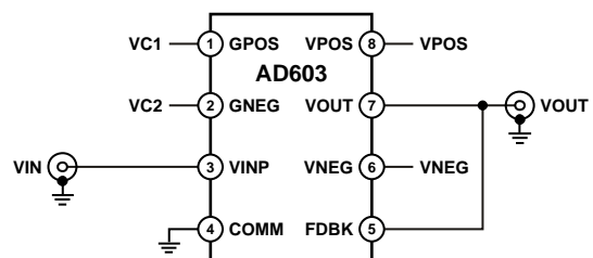
Figure 30. -10 \text{ dB} to +30 \text{ dB} ; 90 MHz Bandwidth
