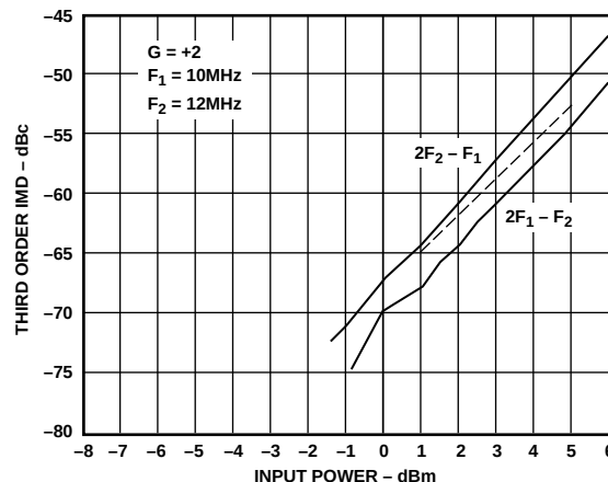
Figure 44. Third Order IMD; F_1 = 10 \text{ MHz} , F_2 = 12 \text{ MHz}
