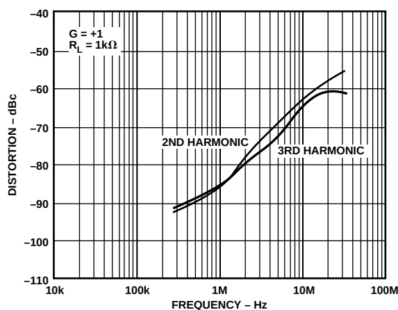
Figure 18. Distortion vs. Frequency, G = +1 , R_L = 1k\Omega
