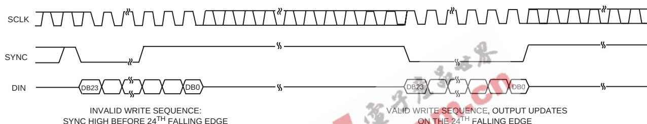
Figure 23. SYNC Interrupt Facility for AD5060.
