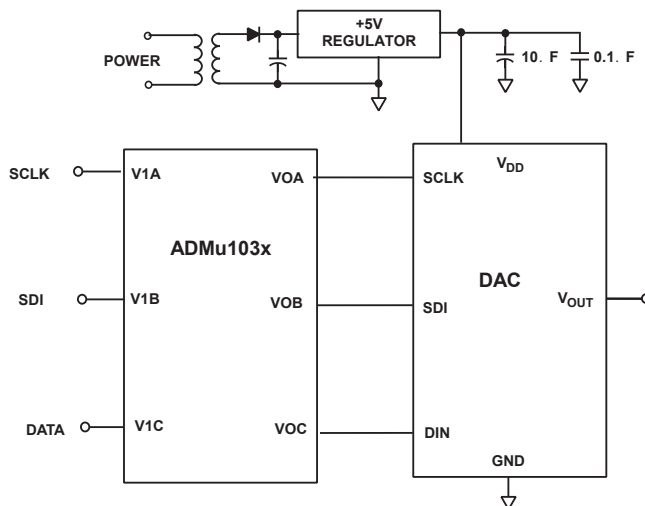
Figure 31. AD5040/AD5060 with An Opto-Isolated Interface
