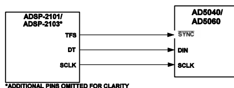
Figure 25. AD5040/AD5060 to ADSP-2101/ADSP-2103 Interface
