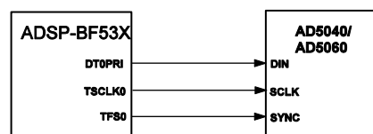
Figure 2X. AD5040/AD5060 to Blackfin ADSP-BF53X Interface
