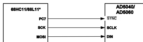
Figure 26. AD5040/AD5060 to 68HC11/68L11 Interface
