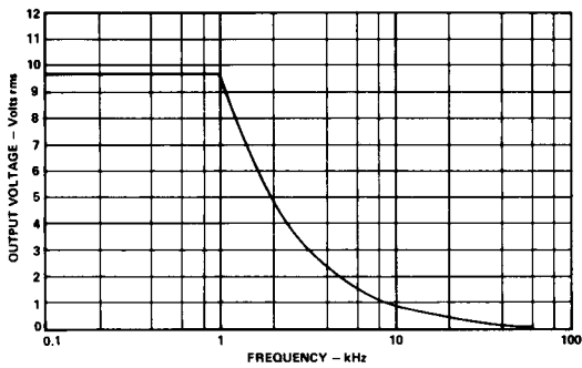
Maximum Undistorted Output vs. Frequency (Distortion ≤ 1%)
