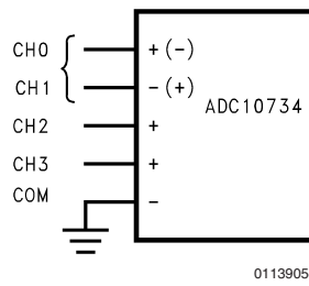
FIGURE 13. Analog Input Multiplexer Options
