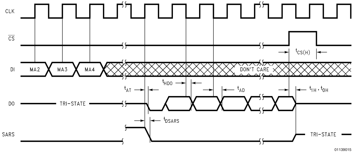
FIGURE 4. DO Timing
