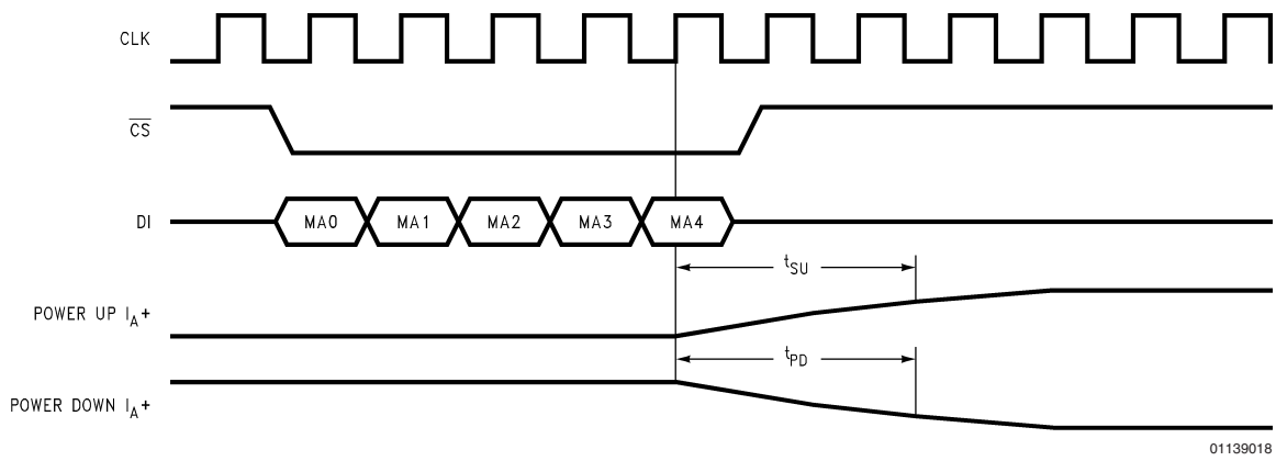
FIGURE 7. Software Power Up/Down Sequence
