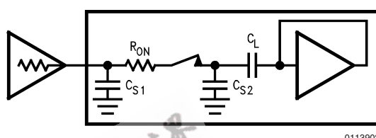
FIGURE 16. Analog Input Model
