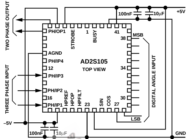
Figure 8. Typical Circuit Configuration
