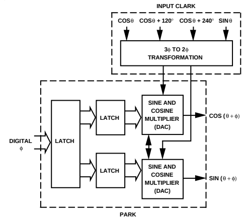
Figure 3. Converter Operation Diagram
