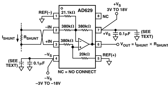
Figure 29. Basic Connections
