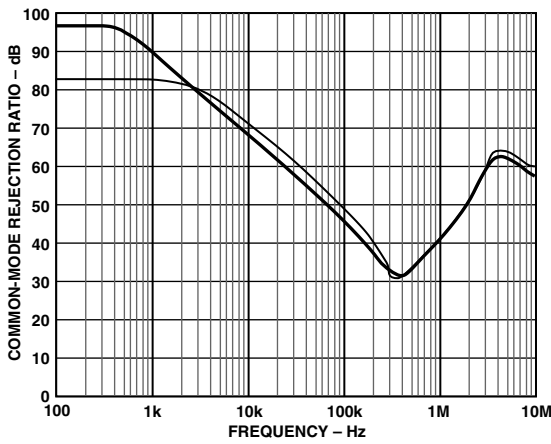
Figure 5. Common-Mode Rejection Ratio vs. Frequency
