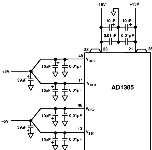
Figure 15. Recommended AD1385 Power Distribution. All 10 \mu\text{F} and 0.01 \mu\text{F} capacitors must have minimum lead length and be located as close as possible to the bypassed pins. Make all ground connections directly to the ground plane.
