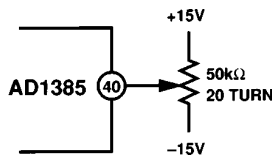
Figure 25a. AD1385 Gain Adjust Circuit
