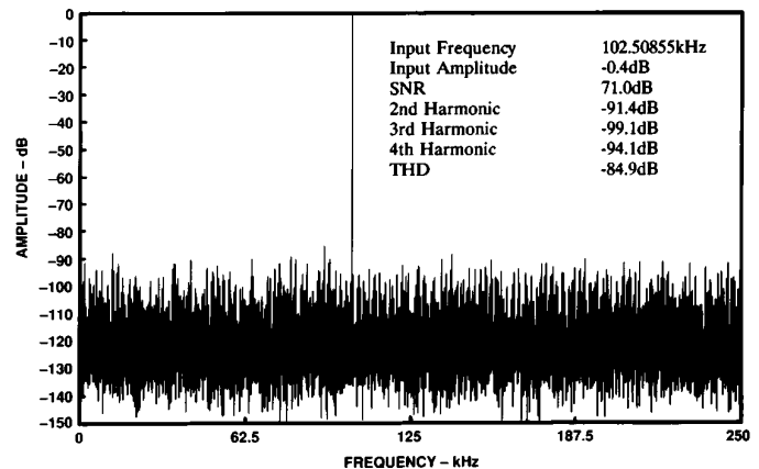
Figure 20. Full-Scale Power Spectral Density after Power-up at T_{CASE} = +25^{\circ}\text{C} Without Calibration, \pm 5 V Range, 16384-Point FFT, 500 kHz Sample Rate. Compare with Figure 4.
