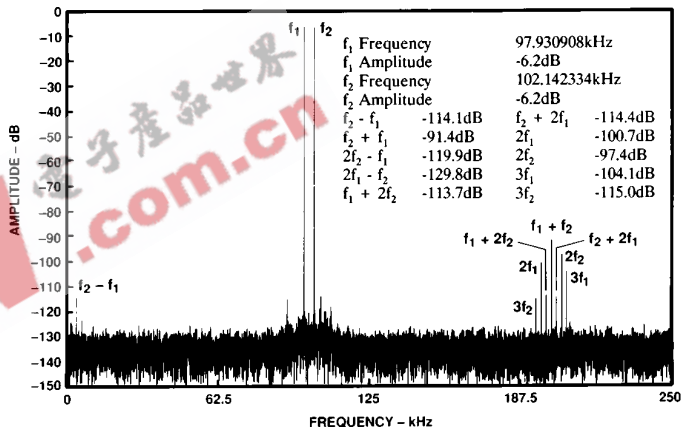
Figure 11. 100 kHz Intermodulation Performance, \pm 10 V Range, 16384-Point FFT, 500 kHz Sample Rate
