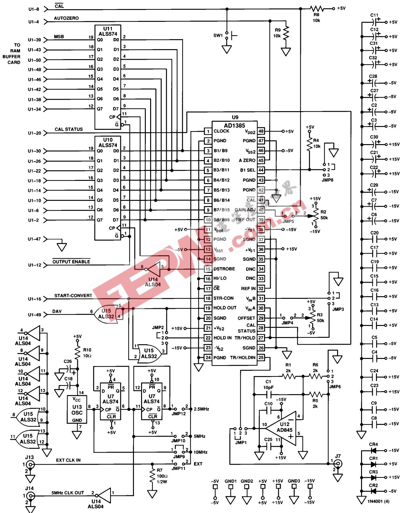
Figure 29. AD1385 Evaluation Board Schematic
