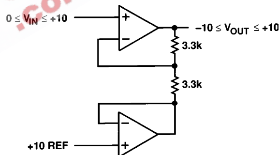
Figure 27. High Input Impedance Unipolar-to-Bipolar Conversion Circuit
