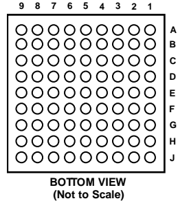
Figure 3. Pin Configuration
