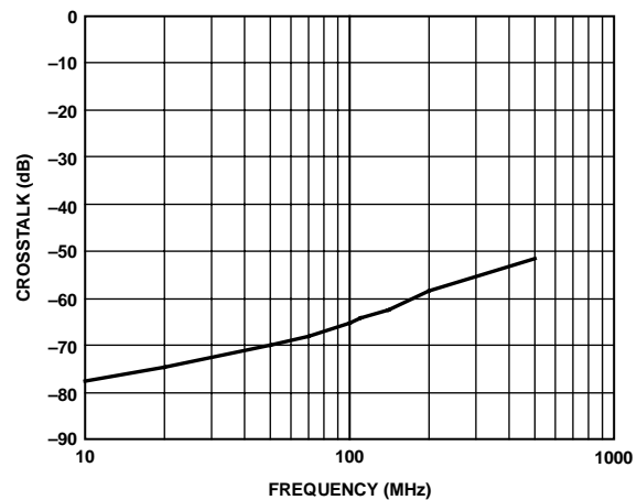
Figure 9. Typical Crosstalk
