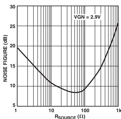
TPC 17. Noise TPC vs. R_{SOURCE}
