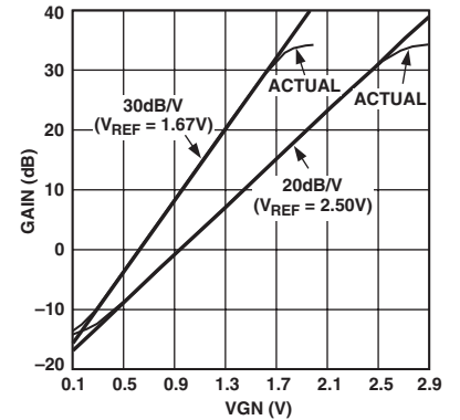
TPC 3. Gain vs. VGN for Different Gain Scalings
