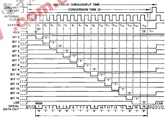
Figure 7. Timing Diagram (Binary Code 0110011101111010)
