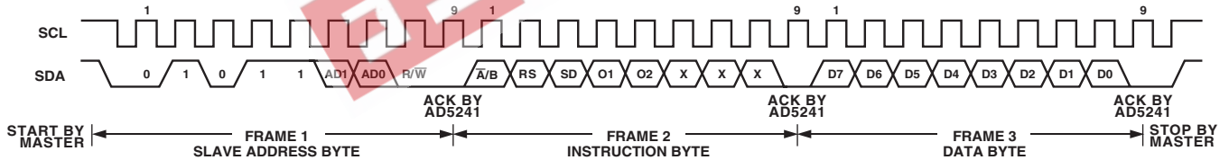
Figure 2. Writing to the RDAC Serial Register
