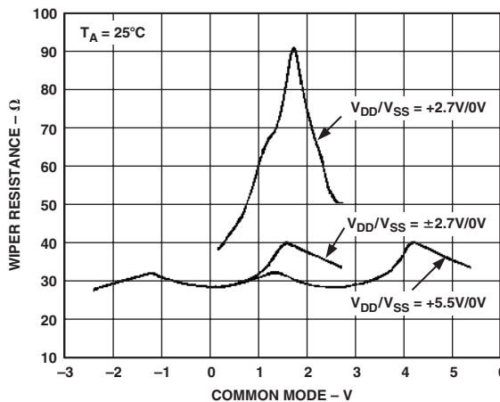
TPC 10. Incremental Wiper Contact vs. V_{DD}/V_{SS}
