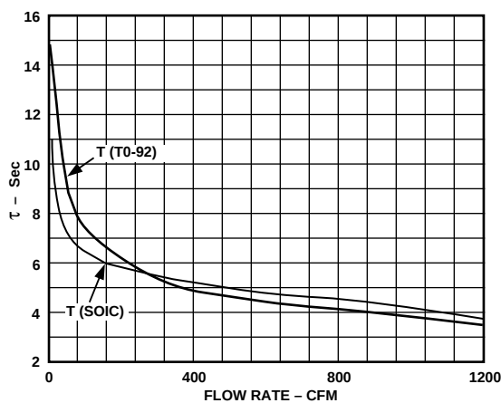
Figure 2. Thermal Response vs. Flow Rate
