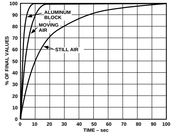
Figure 7. Response Time
