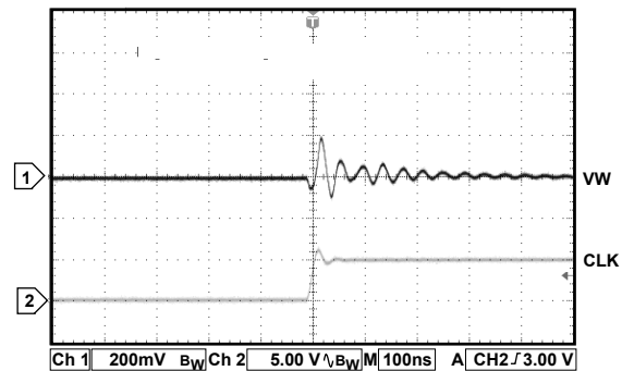
Figure 24. Digital Feedthrough
