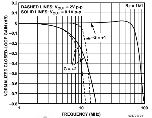
Figure 10. 0.1 dB Flatness Frequency Response
