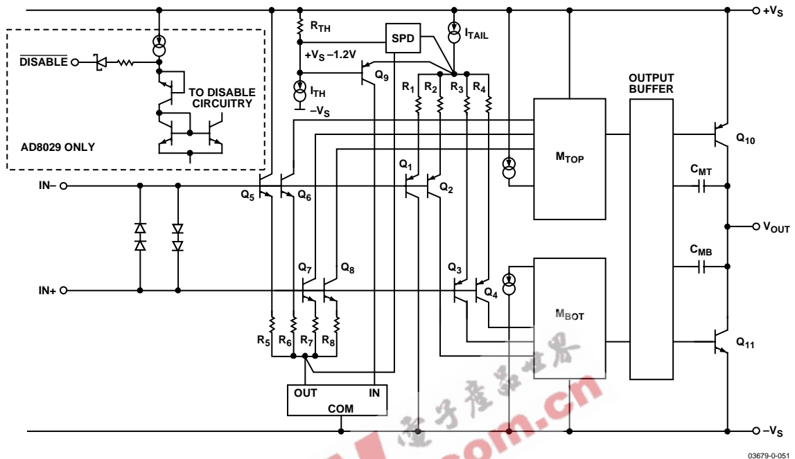
Figure 50. Simplified Schematic
