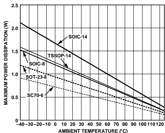
Figure 6. Maximum Power Dissipation
