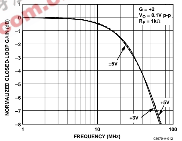
Figure 11. Small Signal Frequency Response for Various Supplies
