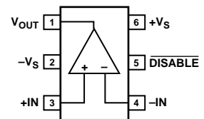
Figure 2. SC70-6 (KS)
