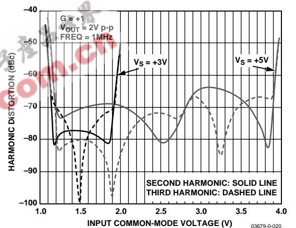
Figure 23. Harmonic Distortion vs. Input Common Mode Voltage
